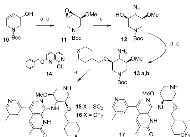
Scheme 1. Conditions: a) m -CPBA, CH 2 Cl 2 , 0 °C; b) NaH, MeI, DMF, 0 °C, 83 % (2 steps); c) LiClO 4 , NaN 3 , CH 3 CN, 80 °C, 35 %; d) tBuOK, THF, 0 °C then RCH 2 OTf, 70–72 %; e) H 2 , Pd/C, MeOH, room temperature, 90–91 %; f) 14 , tBuONa, BrettPhos, Pd(OAc) 2 or Pd(dba) 2 , THF, 60 °C, 37–43 %; g) NBS, CH 2 Cl 2 , –10 °C, 94–97 %; h) ArB(OH) 2 , K 2 CO 3 , Pd(OAc) 2 , cataCXium A, dioxane/H 2 O, microwave, 100 °C, 40–49 %; i) TFA, reflux, > 93 %.
